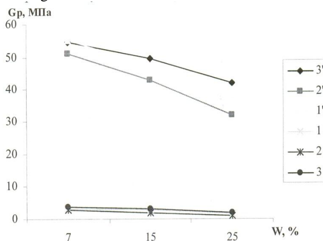
Fig-1. Dependences of the change in the ultimate strength of the soybean husk on its moisture content when breaking along the major axis (1,2 and 3) and along the minor axis (1', 2' and 3') 1-1' Krasnodar variety grown on irrigated lands, 2 and 2' Tashkentskiy variety grown on irrigated lands: 3 and 3' Russian variety grown on irrigated lands
